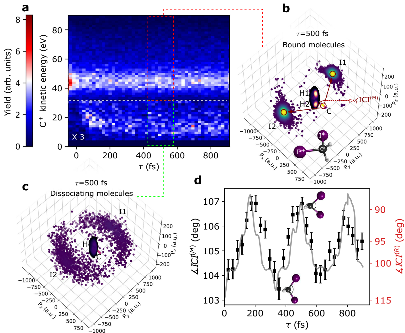
Fig. 2 | Separation of bound and dissociating molecules and imaging of bending vibrations. a Time-dependent KED of C^+ ions for the C^+/I^{3+}/I^{5+} channel. The white dashed line marks the boundary (32 eV) used for separating signals from bound and dissociating molecules. The intensity in the region below the white line is scaled by a factor of 3 to increase the visibility of the dissociation channel. b , c MFMDs for bound ( b ) and dissociating ( c ) molecules (events within the red and green boxes
