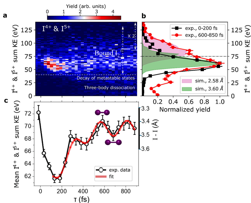
Fig. 3 | Imaging of I_2^+ formation with the C^+/I^{4+}/I^{5+} coincidence channel. a Time-dependent sum KED of I^{4+} and I^{5+} for the events below the white line in Fig. 2a. The horizontal white dashed line in a shows the lower limit (40 eV) of I^{4+} and I^{5+} sum energies associated with bound I_2^+ products. The intensity in the region with KE above 85 eV (marked on the top right) is scaled by a factor of 2 in order to better show the region corresponding to I_2^+ being formed at shorter bond lengths. b Normalized projections of the data in a for 0 < \tau < 200 fs (black) and 600 fs < \tau < 850 fs (red). The error bars were calculated using the Poisson distribution. The black dash-dotted line marks the mean value of the static (“probe-only”) experimental distribution. The shaded areas depict the simulated sum KED for an I-I separation of 2.58 Å (magenta) and 3.60 Å (green). The simulated distributions are normalized such that their respective maxima match the experimental data. c Delay-dependent mean value of the I^{4+} and I^{5+} sum KE, derived from the data above the white dashed line in a . The error bars reflect the standard error of the mean. The data are fitted with the sum of an error function and a sinusoidal function with 250 fs period. The right axis shows the internuclear separations of the formed I_2^+ product for which our simulations yield the mean values of the I^{4+} and I^{5+} sum KEs shown on the left axis.
